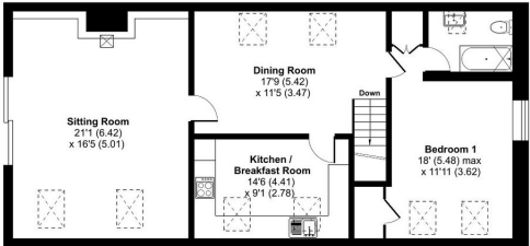
FIRST FLOOR
